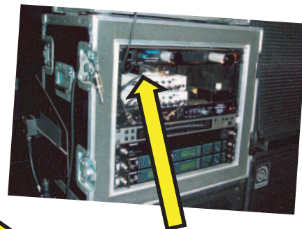
John McVie's Bass Rig: Great Tone - No Hum! Left: Ebtech® HE-8 Hum Eliminator Right: Ebtech® HE-2 Hum Eliminator
